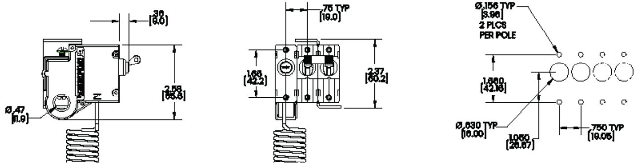
TYPICAL 2-POLE 120/240 VAC VERSION
