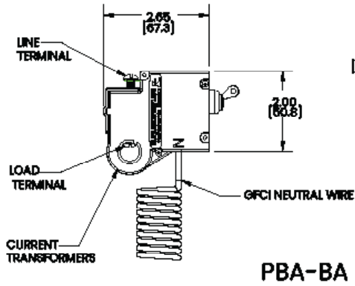
TYPICAL 2-POLE 120/240 VAC VERSION
