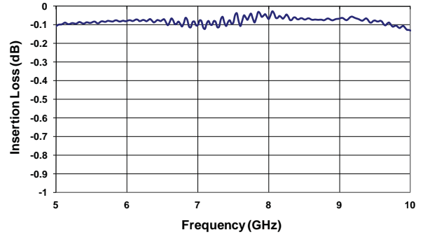
Insertion Loss (5-10 GHz)
