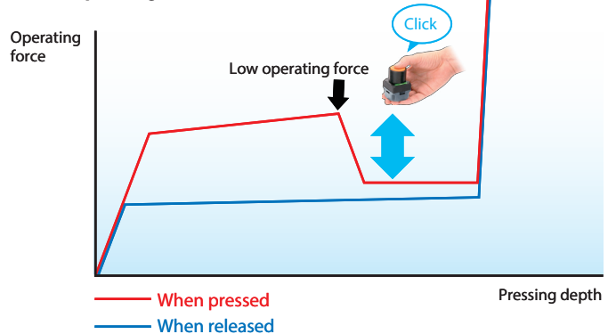
Relationship between pressing depth and operating force
