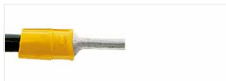
Crimped pin terminal (gas-tight), preferably made of copper with a tin-plated surface
