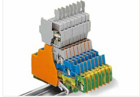
When triple-deck terminal blocks are used with a fuse plug (6 mm wide) in the receptacle (top) level, the extra width can be compensated for the 280 Series (5 mm wide) via an intermediate plate (1.1 mm thick).
