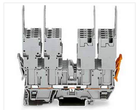
4-pin carrier terminal block (769-151)
