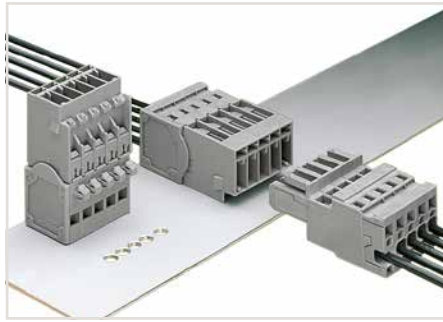
Male connector; with CAGE CLAMP® connection and snap-in mounting feet 1-conductor female plug; straight
