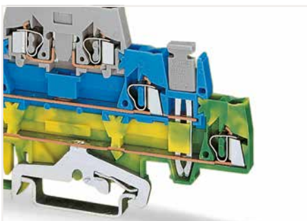
Grounding to DIN-rail: Connecting N-level to ground level via vertical jumper.
