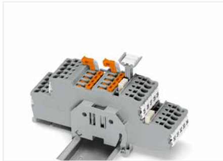
Double-deck, double-disconnect terminal blocks (2002-2951) with group marker carrier (2002-160) accommodated in jumper contact slot
