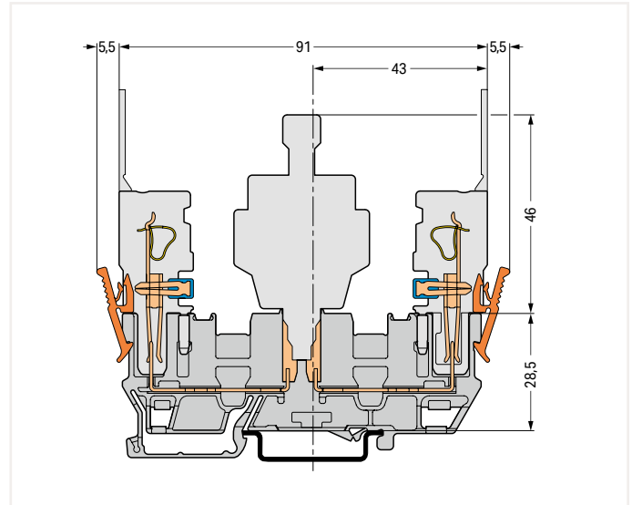
Carrier terminal block For other dimensions, see carrier terminal block (769-151).
