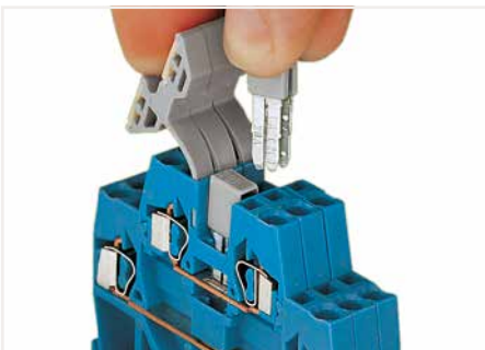
Commoning using an adjacent jumper (280-402). push jumpers down until fully inserted.
