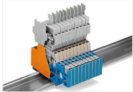
When double-deck terminal blocks are used with a fuse plug (6 mm wide) in the receptacle (top) level, the extra width can be compensated for the 280 Series (5 mm wide) via an intermediate plate (1.1 mm thick). If required, this special intermediate plate still allows commoning on the lower level via push-in adjacent jumpers (280-402).
