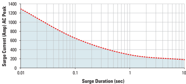
DR2260x35x
