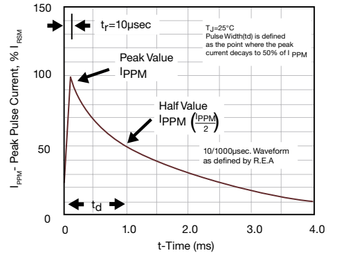
Figure 3 - Pulse Waveform
