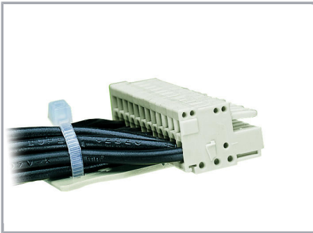
Strain relief plate, for factory assembly
