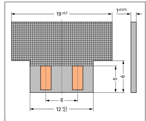
Dimensions of self-assembled PCBs:
