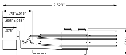
Three-Conductor Single Bantam Jack
