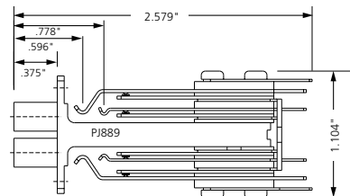
Three-Conductor Dual Bantam Jack
