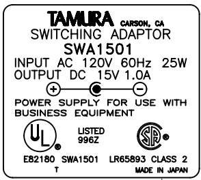
NAMEPLATE TOP CASE (SCALE:1/1)
