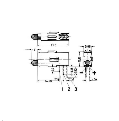
1, 2, 3 = mounting planes
