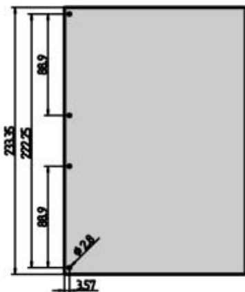
Drill hole dimensions on PCB, 3 U
