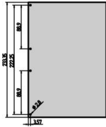
Drill hole dimensions on PCB, 6 U
