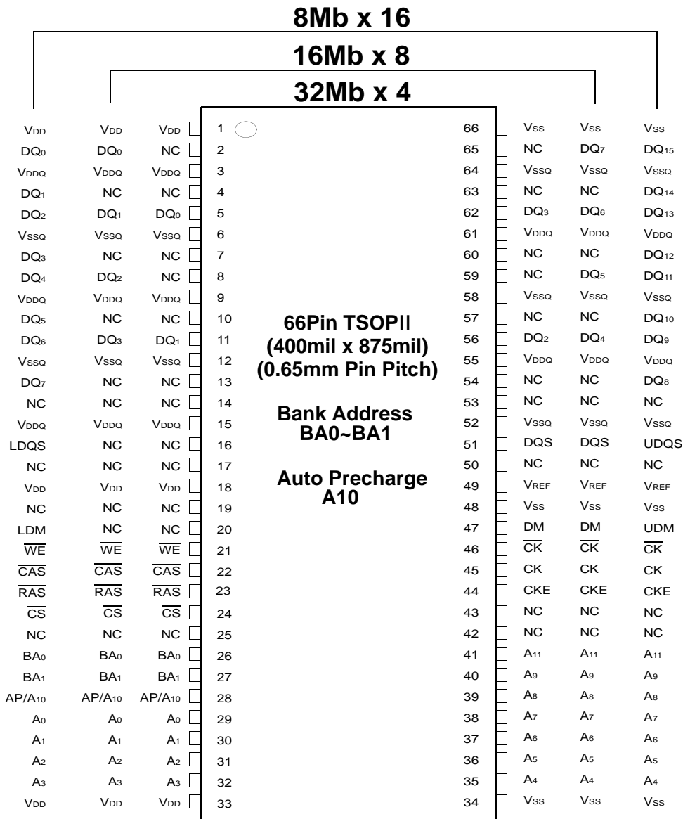
128Mb Package Pinout
