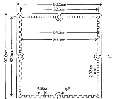
Enclosure Profile
