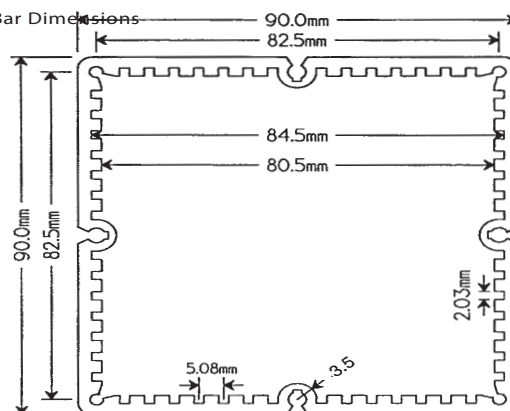
Housing Profile and Mounting Bar Dimensions
