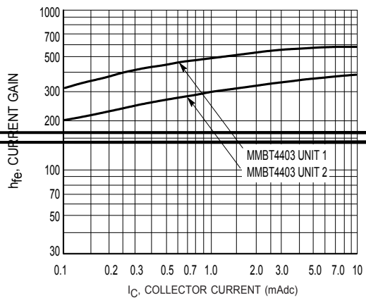
Figure 8. Current Gain
