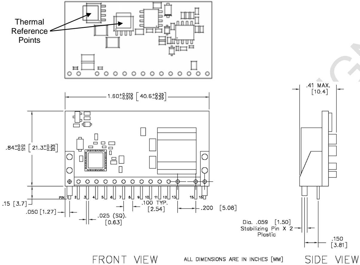
Figure 14. Mechanical Drawing
