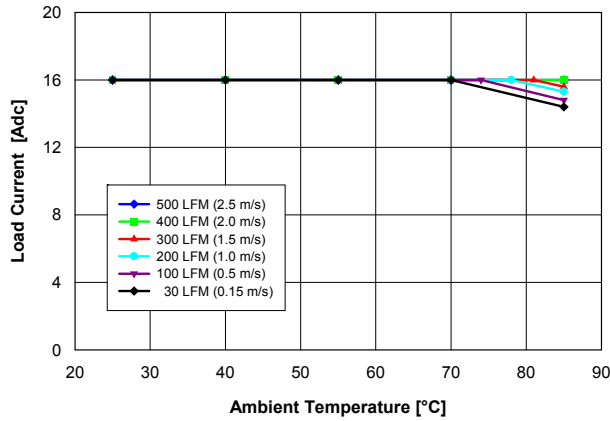
Fig. 2.5V.1: Available load current vs. ambient temperature and airflow rates for Vout = 2.5V converter mounted vertically with Vin = 12V, and maximum MOSFET temperature ≤ 120°C.
