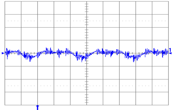
Fig. 1.2V.6: Output voltage ripple (20 mV/div.) at full rated load current into a resistive load with external capacitance 47\ \mu\text{F} ceramic + 1\ \mu\text{F} ceramic, and V_{in} = 5\text{ V} for V_{out} = 1.2\text{ V} . Time scale: 2 \mu\text{s} /div.
