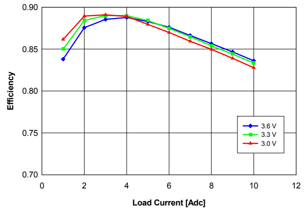
Fig. 0.7525V.4: Efficiency vs. load current and input voltage for V_{out} = 0.7525\text{ V} converter mounted horizontally with air flowing at a rate of 200 LFM (1 m/s) and T_a = 25\text{ }^{\circ}\text{C} .
