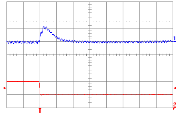
Fig. 2.5V.8: Output voltage response (YNL05S10025) to negative load current step change from 10 A to 5 A with slew rate of -5 \text{A}/\mu\text{s} at V_{in} = 5\text{ V} . Top trace: output voltage (100 mV/div.); Bottom trace: load current (5 A/div.). C_o = 47\ \mu\text{F} ceramic + 1 \mu\text{F} ceramic. Time scale: 20 \mu\text{s} /div.
