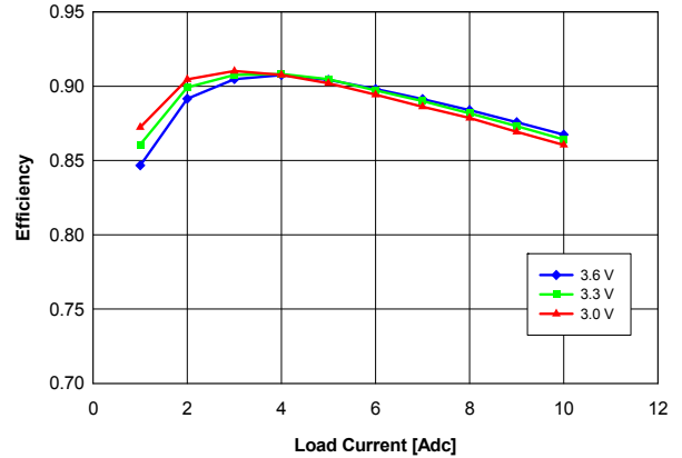
Fig. 1.0V.4: Efficiency vs. load current and input voltage for YNL05S10010 converter mounted vertically with air flowing at a rate of 200 LFM (1 m/s) and T_a = 25\text{ }^{\circ}\text{C} .
