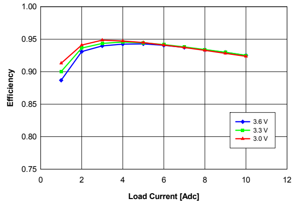
Fig. 2.0V.4: Efficiency vs. load current and input voltage for YNL05S10020 converter mounted vertically with air flowing at a rate of 200 LFM (1 m/s) and T_a = 25\text{ }^{\circ}\text{C} .
