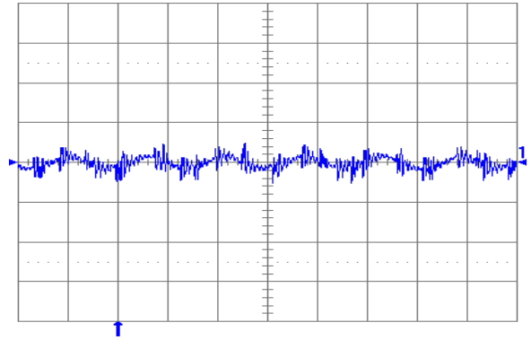
Fig. 1.8V.6: Output voltage ripple (20 mV/div.) at full rated current into a resistive load with external capacitance 47 \mu\text{F} ceramic + 1 \mu\text{F} ceramic and V_{in} = 5\text{ V} (YNL05S10018). Time scale: 2 \mu\text{s} /div.
