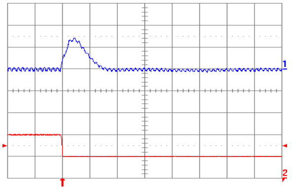
Fig. 1.8V.8: Output voltage response (YNL05S10018) to negative load current step change from 10 A to 5 A with slew rate of -5 A/ \mu\text{s} at V_{in} = 5\text{ V} . Top trace: output voltage (100 mV/div.); Bottom trace: load current (5 A/div.). C_o = 47\ \mu\text{F} ceramic + 1 \mu\text{F} ceramic. Time scale: 20 \mu\text{s} /div.
