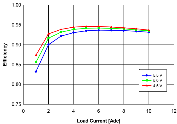
Fig. 2.5V.3: Efficiency vs. load current and input voltage for YNL05S10025 converter mounted vertically with air flowing at a rate of 200 LFM (1 m/s) and T_a = 25\text{ }^{\circ}\text{C} .
