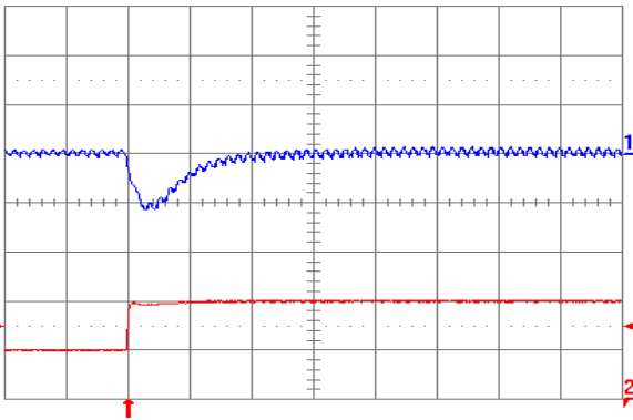
Fig. 1.8V.7: Output voltage response (YNL05S10018) to positive load current step change from 5 A to 10 A with slew rate of 5 A/ \mu\text{s} at V_{in} = 5\text{ V} . Top trace: output voltage (100 mV/div.); Bottom trace: load current (5 A/div.). C_o = 47\ \mu\text{F} ceramic + 1 \mu\text{F} ceramic. Time scale: 20 \mu\text{s} /div.
