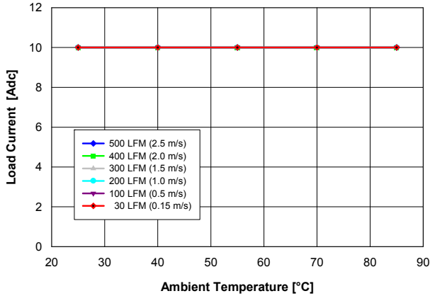
Fig. 2.0V.1: Available load current vs. ambient temperature and airflow rates for YNL05S10020 converter mounted vertically with V_{in} = 5\text{ V} , and maximum MOSFET temperature \leq 110\text{ }^{\circ}\text{C} .
