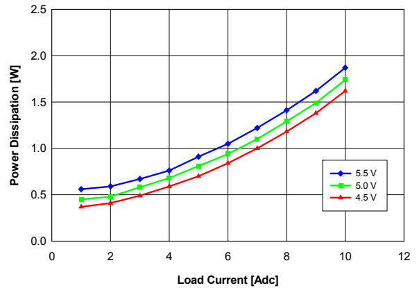
Fig. 3.3V.4: Power Loss vs. load current and input voltage for YNL05S10033 converter mounted vertically with air flowing at a rate of 200 LFM (1 m/s) and T_a = 25\text{ }^{\circ}\text{C} .
