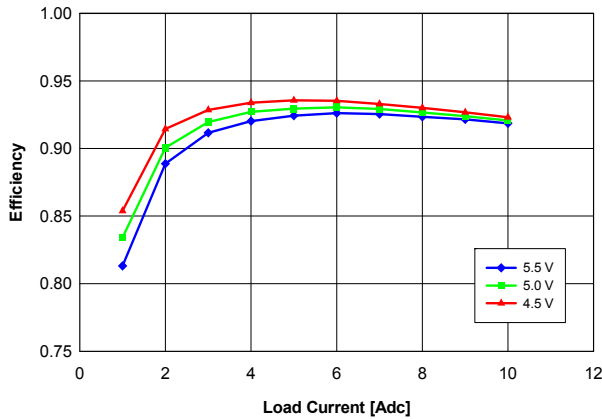
Fig. 2.0V.3: Efficiency vs. load current and input voltage for YNL05S10020 converter mounted vertically with air flowing at a rate of 200 LFM (1 m/s) and T_a = 25\text{ }^{\circ}\text{C} .
