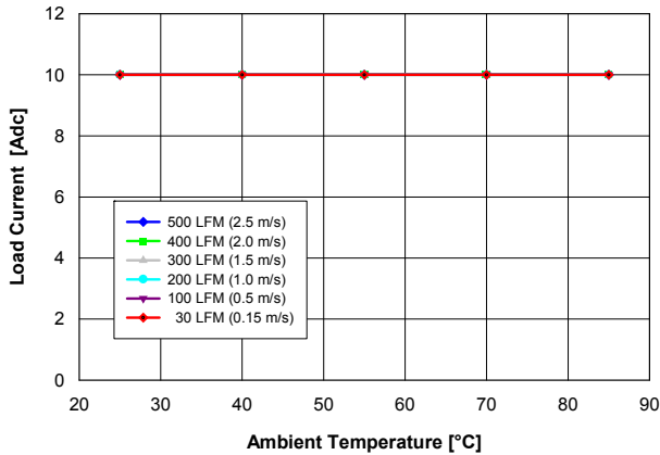
Fig. 1.8V.1: Available load current vs. ambient temperature and airflow rates for YNL05S10018 converter mounted vertically with Vin = 5 V, and maximum MOSFET temperature ≤ 110 °C.
