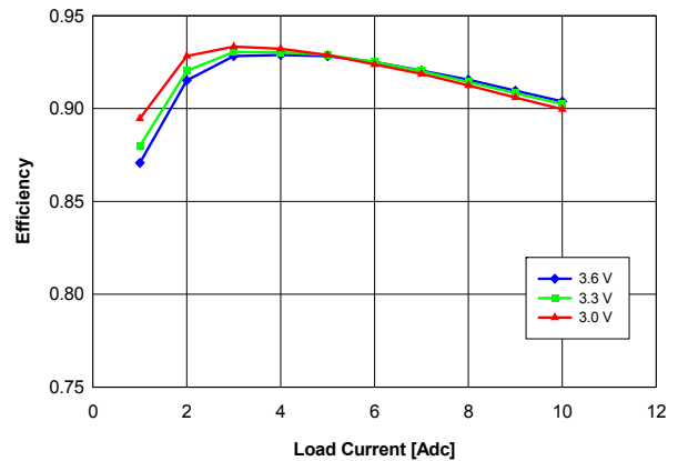
Fig. 1.5V.4: Efficiency vs. load current and input voltage for YNL05S10015 converter mounted vertically with air flowing at a rate of 200 LFM (1 m/s) and T_a = 25\text{ }^{\circ}\text{C} .
