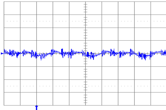
Fig. 1.0V.6: Output voltage ripple (20 mV/div.) at full rated load current into a resistive load with external capacitance 47 \mu F ceramic + 1 \mu F ceramic and V_{in} = 5 V (YNL05S10010). Time scale: 2 \mu s/div.
