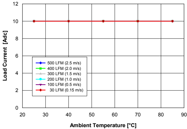
Fig. 2.5V.1: Available load current vs. ambient temperature and airflow rates for YNL05S10025 converter mounted vertically with V_{in} = 5\text{ V} , and maximum MOSFET temperature \leq 110\text{ }^{\circ}\text{C} .
