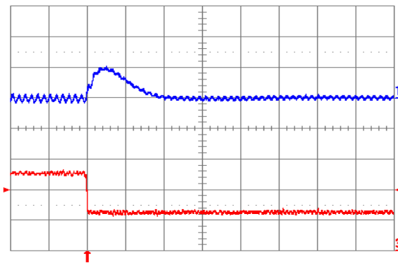
Fig. 1.0V.8: Output voltage response (YNL05S10010) to negative load current step change from 10 A to 5 A with slew rate of -5 A/ \mu s at V_{in} = 5 V. Top trace: output voltage (100 mV/div.); Bottom trace: load current (5 A/div.). C_o = 47 \mu F ceramic + 1 \mu F ceramic. Time scale: 20 \mu s/div.
