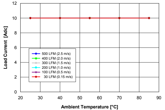
Fig. 1.5V.2: Available load current vs. ambient temperature and airflow rates for YNL05S10015 converter mounted horizontally with V_{in} = 5\text{ V} , and maximum MOSFET temperature \leq 110\text{ }^{\circ}\text{C} .
