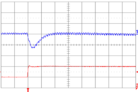
Fig. 1.2V.7: Output voltage response (YNL05S10012) to positive load current step change from 5 A to 10 A with slew rate of 5 A/ \mu\text{s} at V_{in} = 5\text{ V} . Top trace: output voltage (100 mV/div.); Bottom trace: load current (5 A/div.). C_o = 47\ \mu\text{F} ceramic + 1 \mu\text{F} ceramic. Time scale: 20 \mu\text{s} /div.
