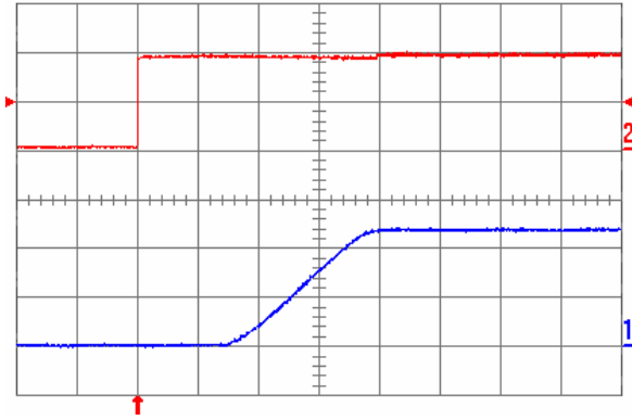
Fig. 1.2V.5: Turn-on transient (YNL05S10012) with the application of Enable signal at full rated load current (resistive) and 47 \mu\text{F} external capacitance at V_{in} = 5\text{ V} . Top trace: Enable signal (2 V/div.); Bottom trace: output voltage (500 mV/div.); Time scale: 2 ms/div.
