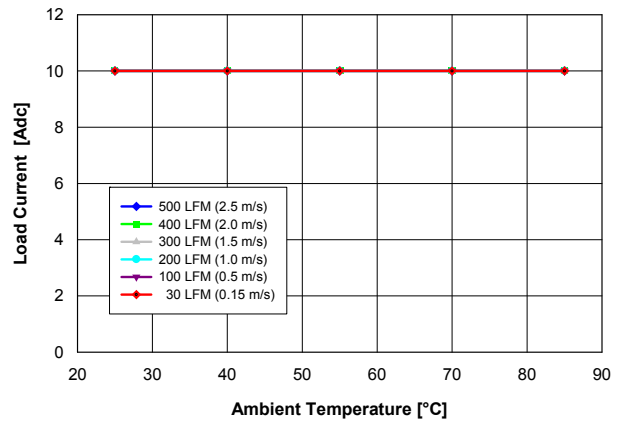
Fig. 1.8V.2: Available load current vs. ambient temperature and airflow rates for YNL05S10018 converter mounted horizontally with Vin = 5 V, and maximum MOSFET temperature ≤ 110 °C.
