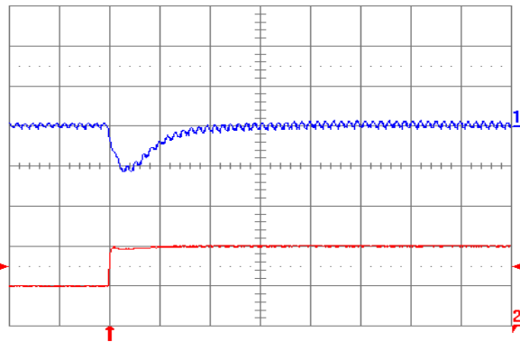
Fig. 2.0V.7: Output voltage response (YNL05S10020) to positive load current step change from 5 A to 10 A with slew rate of 5 A/ \mu s at V_{in} = 5 V. Top trace: output voltage (100 mV/div.); Bottom trace: load current (5 A/div.). C_o = 47 \mu F ceramic + 1 \mu F ceramic. Time scale: 20 \mu s/div.
