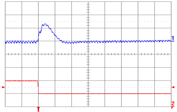
Fig. 1.2V.8: Output voltage response (YNL05S10012) to negative load current step change from 10 A to 5 A with slew rate of -5 A/ \mu\text{s} at V_{in} = 5\text{ V} . Top trace: output voltage (100 mV/div.); Bottom trace: load current (5 A/div.). C_o = 47\ \mu\text{F} ceramic + 1 \mu\text{F} ceramic. Time scale: 20 \mu\text{s} /div.
