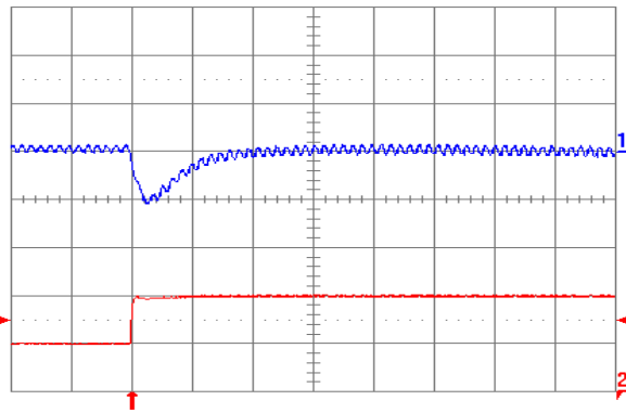
Fig. 2.5V.7: Output voltage response (YNL05S10025) to positive load current step change from 5 A to 10 A with slew rate of 5 \text{A}/\mu\text{s} at V_{in} = 5\text{ V} . Top trace: output voltage (100 mV/div.); Bottom trace: load current (5 A/div.). C_o = 47\ \mu\text{F} ceramic + 1 \mu\text{F} ceramic. Time scale: 20 \mu\text{s} /div.
