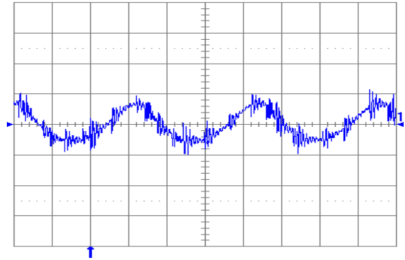
Fig. 3.3V.6: Output voltage ripple (20 mV/div.) at full rated load current into a resistive load with external capacitance 47 \mu F ceramic + 1 \mu F ceramic and V_{in} = 5 V (YNL05S10033). Time scale: 2 \mu s/div.
