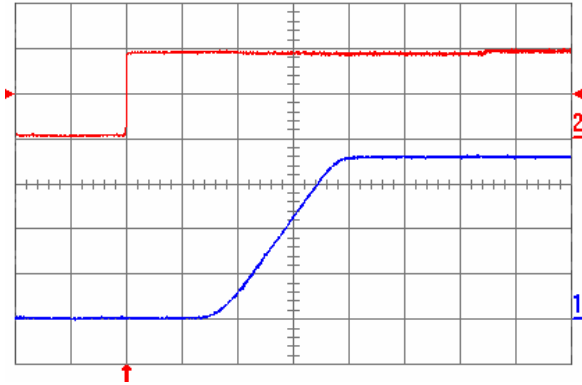
Fig. 1.8V.5: Turn-on transient (YNL05S10018) with the application of Enable signal at full rated load current (resistive) and 47 \mu\text{F} external capacitance at V_{in} = 5\text{ V} . Top trace: Enable signal (2 V/div.); Bottom trace: output voltage (500 mV/div.); Time scale: 2 ms/div.
