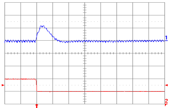
Fig. 1.5V.8: Output voltage response (YNL05S10015) to negative load current step change from 10 A to 5 A with slew rate of -5 A/ \mu\text{s} at V_{in} = 5\text{ V} . Top trace: output voltage (100 mV/div.); Bottom trace: load current (5 A/div.). C_o = 47\ \mu\text{F} ceramic + 1 \mu\text{F} ceramic. Time scale: 20 \mu\text{s} /div.
