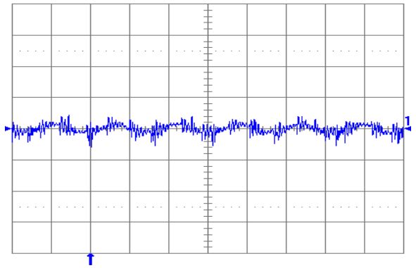
Fig. 1.5V.6: Output voltage ripple (20 mV/div.) at full rated load current into a resistive load with external capacitance 47 \mu\text{F} ceramic + 1 \mu\text{F} ceramic and V_{in} = 5\text{ V} (YNL05S10015). Time scale: 2 \mu\text{s} /div.
