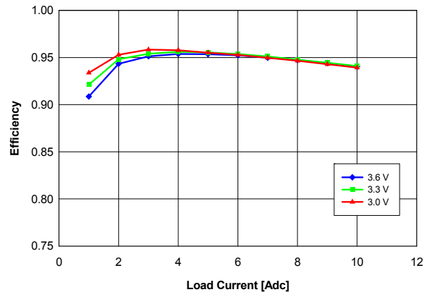
Fig. 2.5V.4: Efficiency vs. load current and input voltage for YNL05S10025 converter mounted vertically with air flowing at a rate of 200 LFM (1 m/s) and T_a = 25\text{ }^{\circ}\text{C} .
