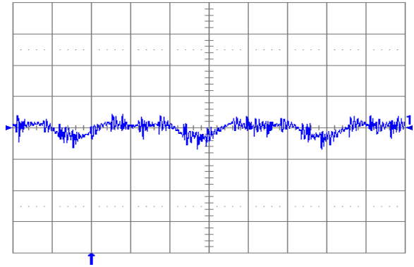
Fig. 1.2V.6: Output voltage ripple (20 mV/div.) at full rated load current into a resistive load with external capacitance 47 \mu\text{F} ceramic + 1 \mu\text{F} ceramic and V_{in} = 5\text{ V} (YNL05S10012). Time scale: 2 \mu\text{s} /div.
