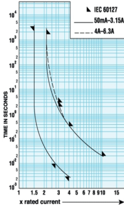
Time-Current Graph: International 5x20mm Fuse Quick-Acting • High Breaking Capacity
