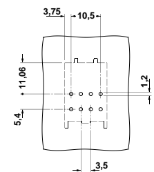
Drilling diagram VC-AMLV 8
