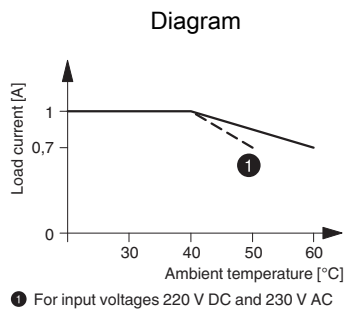
The figure shows the derating curve for PLC-...300DC/1
