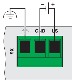
Connection diagram
