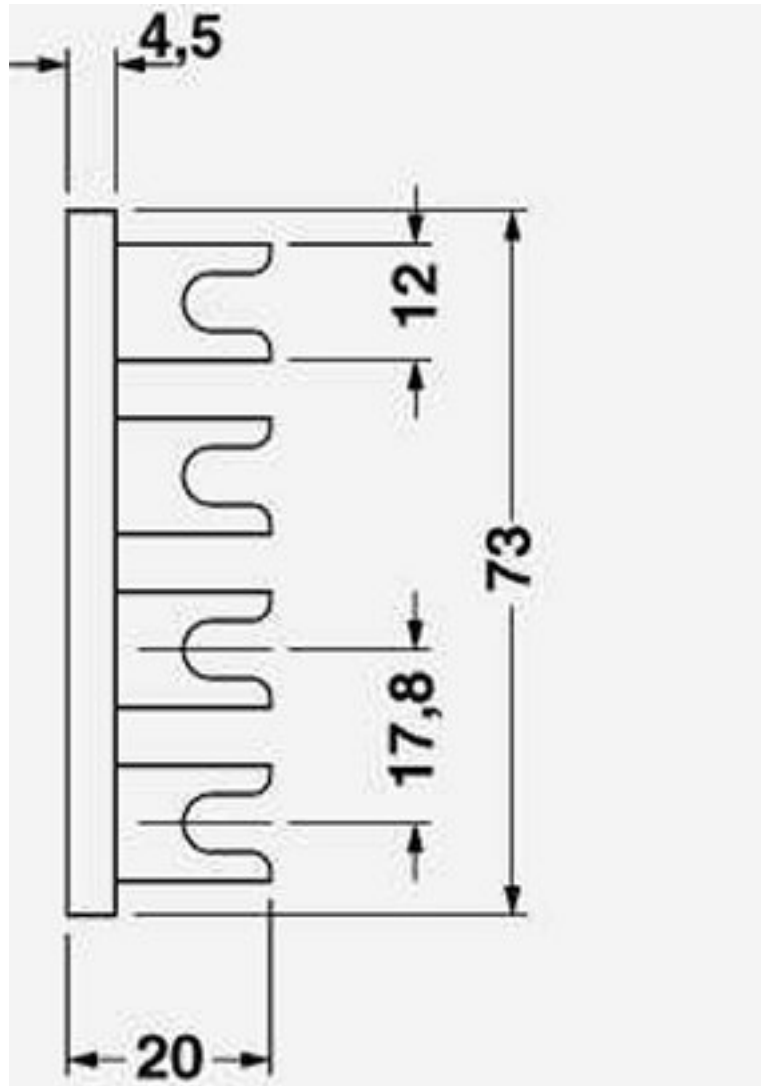
Dimensional drawing
