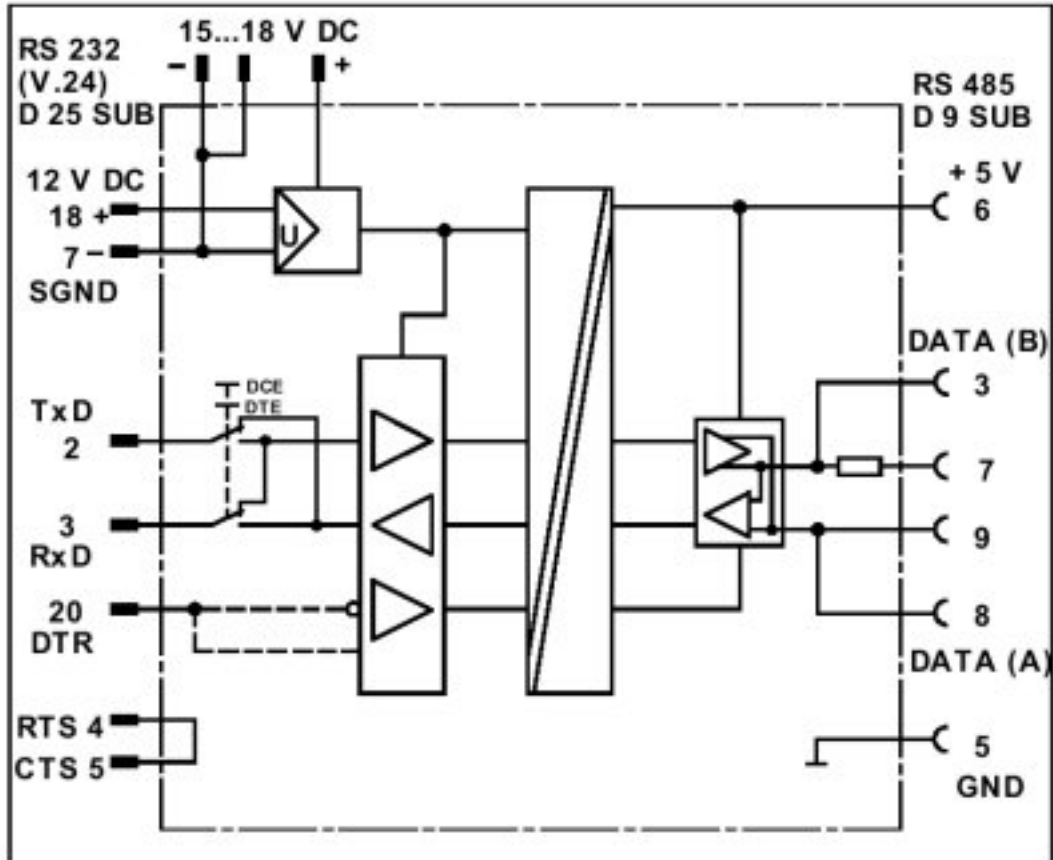
Circuit diagram
