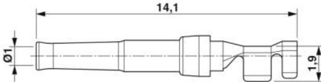
Dimensional drawing
