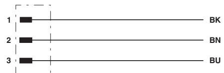
Contact assignment of 7/8" plug
