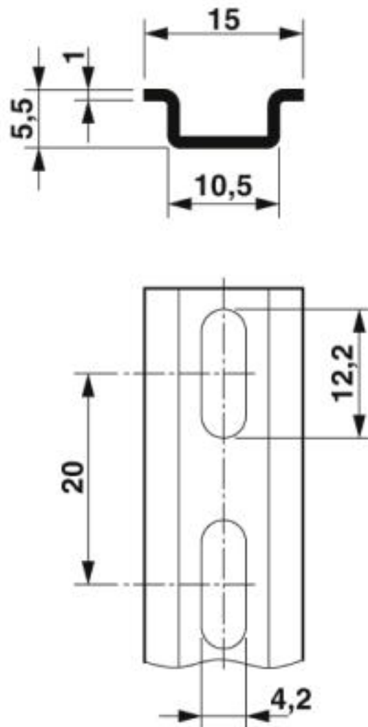
Dimensional drawing
