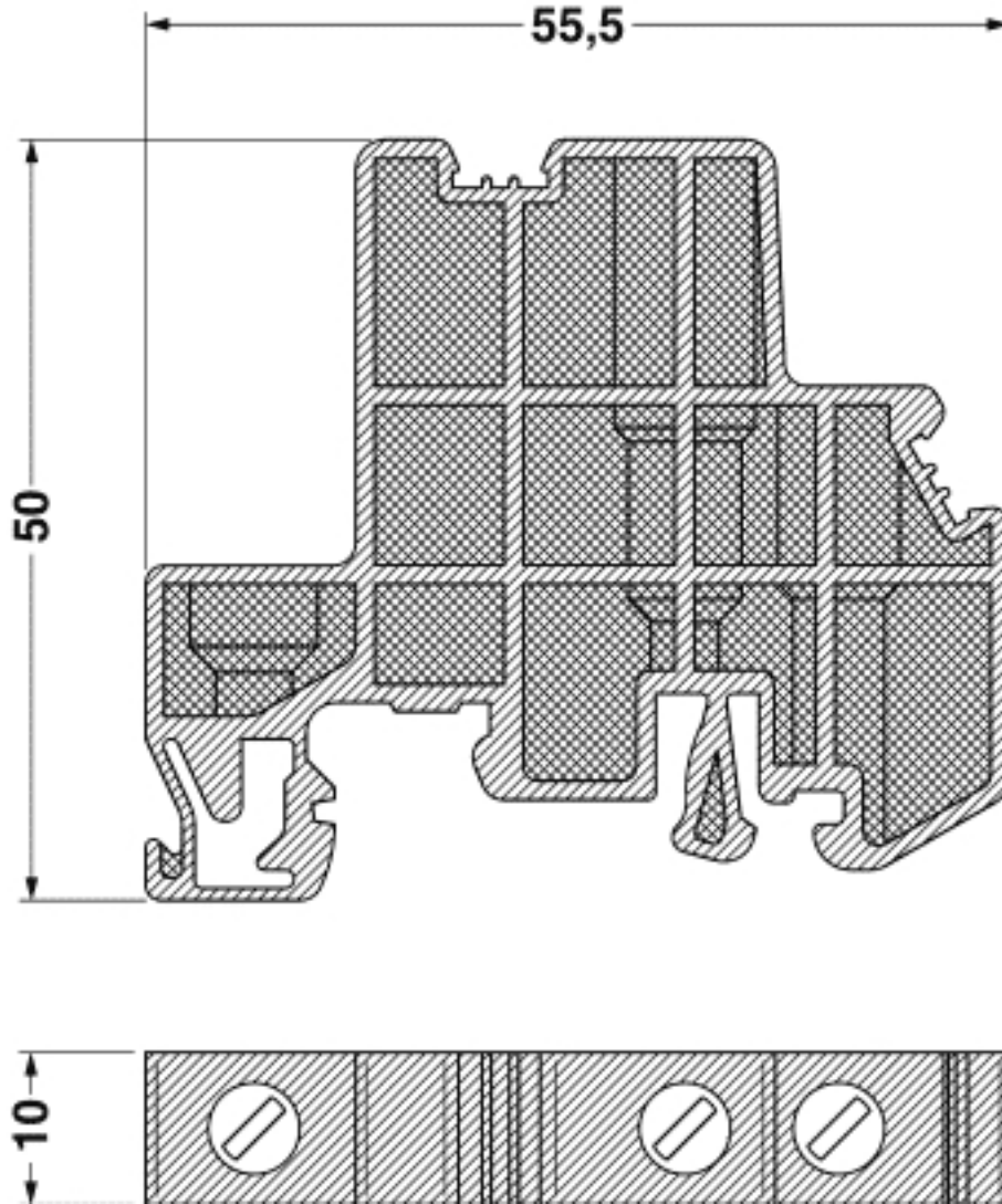
Dimensional drawing
