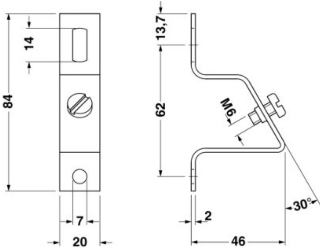
Dimensional drawing
