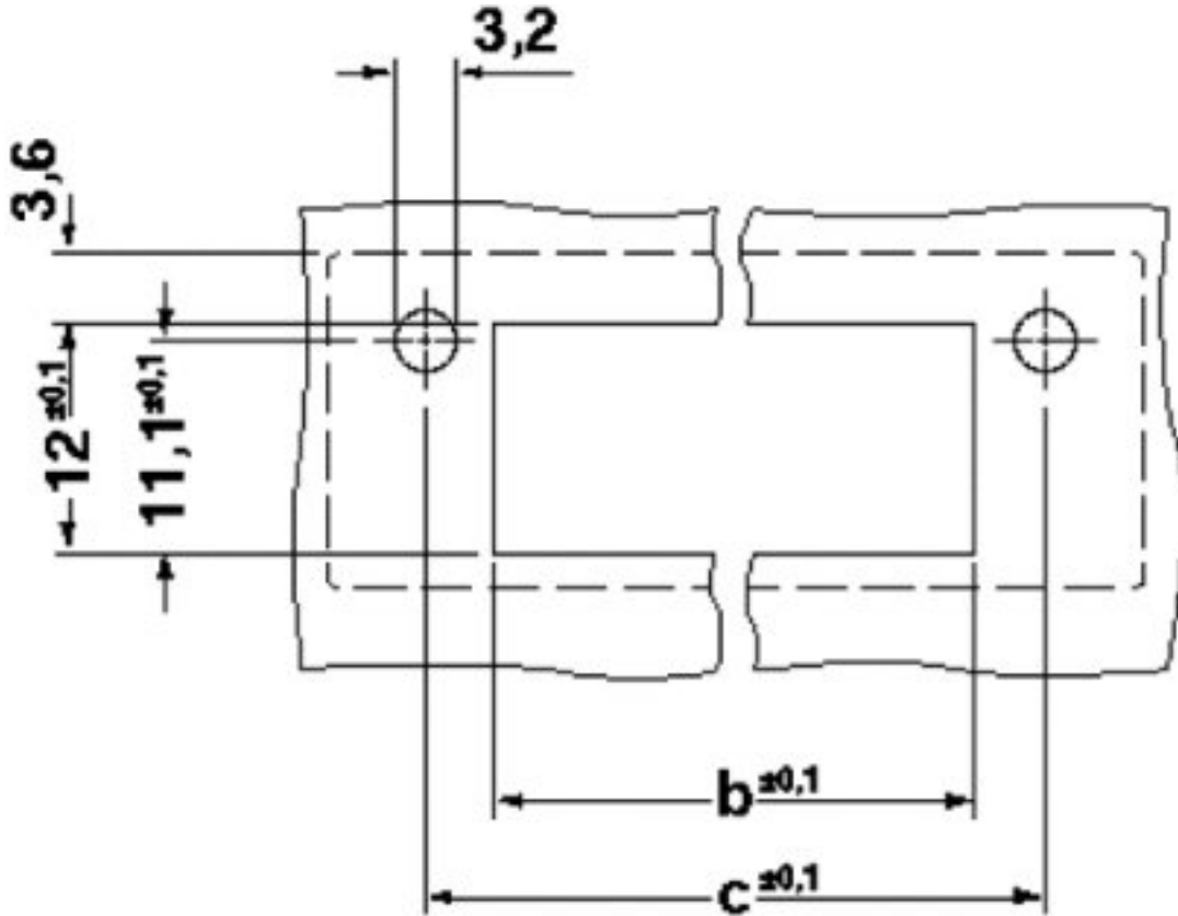
Drilling diagram
