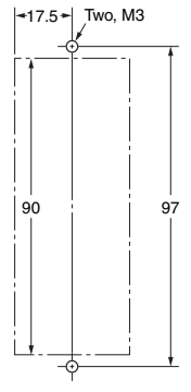
Mounting Hole Dimensions
