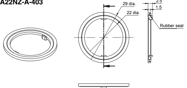
Lock Ring A22NZ-A-403
