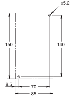
Mounting dimensions
