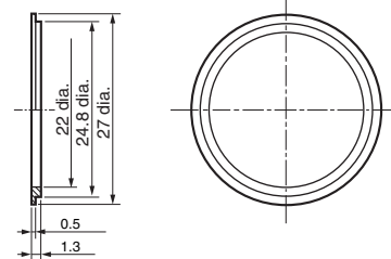
Incandescent Lamp A22-5, 12, 24, H1
