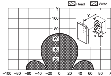
V680-HS63 (mounted on metallic material) & V680-D8KF68/-D32KF68 (mounted on metallic surface: steel) (Tag direction: Vertical) When the V680-A81 attachment is mounted on RF Tag
