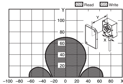
V680-HS63 (mounted on metallic material) & V680-D8KF68/-D32KF68 (mounted on metallic surface: steel) (Tag direction: Vertical)
