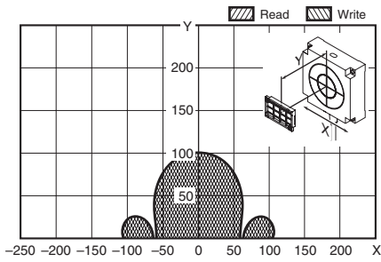
V680-HS65 (with Metal on Back Surface) & V680S-DKF68 (Metal on back: Steel) (Tag direction: Horizontal)
