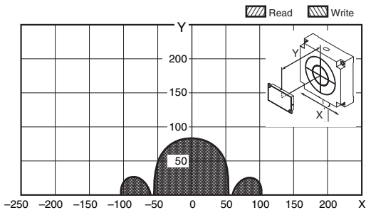
V680-HS65 (mounted on metallic material) & V680-D8KF68/-D32KF68 (flush-mounted on metallic surface: steel) (Tag direction: Horizontal) When the V680-A81 attachment is mounted on RF Tag
