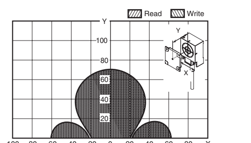
V680-H01-V2 (mounted on non-metallic material) & V680S-D2KF67 (mounted on non-metallic material)
