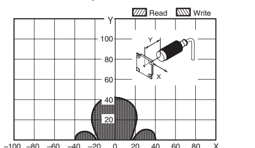
V680-HS65 (mounted on metallic material) & V680S-D2KF67 (mounted on non-metallic material)
