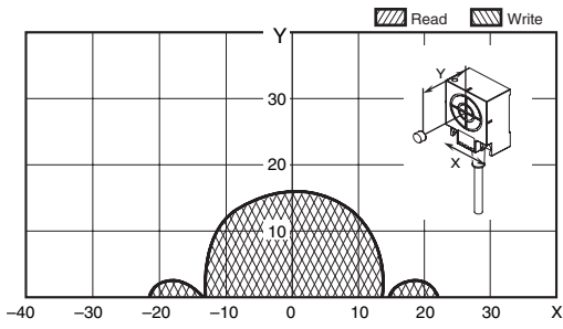
V680-HS63 (mounted on non-metallic material) & V680S-D2KF67 (mounted on non-metallic material)
