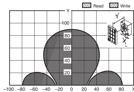
V680-HS63 (with Metal on Back Surface) & V680S-D2KF68 (Tag direction: Vertical)
