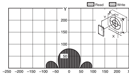
V680-HS65 (mounted on metallic material) & V680-D8KF68/-D32KF68 (flush-mounted on metallic surface: steel) (Tag direction: Vertical) When the V680-A81 attachment is mounted on RF Tag
