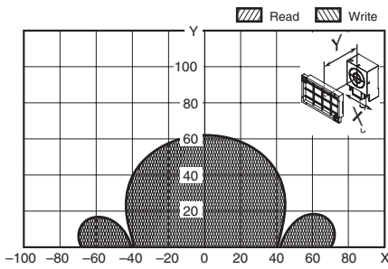
V680-HS65 (with Metal on Back Surface) & V680S-D2KF68M (Metal on back: Steel) (Tag direction: Horizontal)
