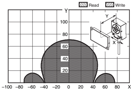
V680-HS63 (mounted on metallic material) & V680-D8KF68/-D32KF68 (mounted on metallic surface: steel) (Tag direction: Horizontal)
