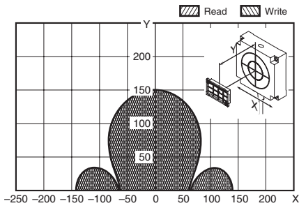
V680-HS63 (with Metal on Back Surface) & V680S-D2KF68M (Metal on back: Steel) (Tag direction: Horizontal)
