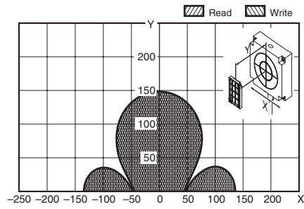
V680-HS63 (with Metal on Back Surface) & V680S-D2KF68M (Metal on back: Steel) (Tag direction: Vertical)
