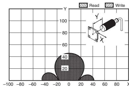
V680-HS65 (mounted on metallic material) & V680S-D2KF67 (mounted on non-metallic material)
