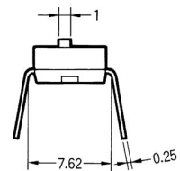
Raised Actuator
