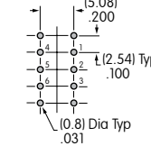
Momentary & Alternate
