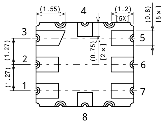
Fig.2 Package dimensions (in mm)
