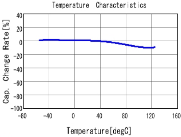
■ GRM188R71C104KA01 C-Temp. capchange, DC0.0V, AC1.0V rm
