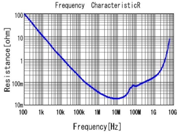
■ GRM188R71C104KA01 R DCOV, 25degC
