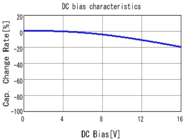
■ GRM188R71C104KA01 C-DC bias capchange, 25.0degC, AC1.
