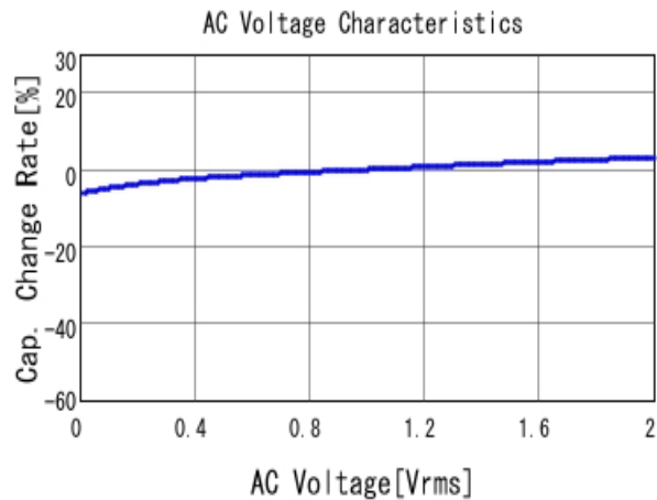
■ GRM188R71C104KA01 C-AC Voltage capchange, DCOV, 25.0d
