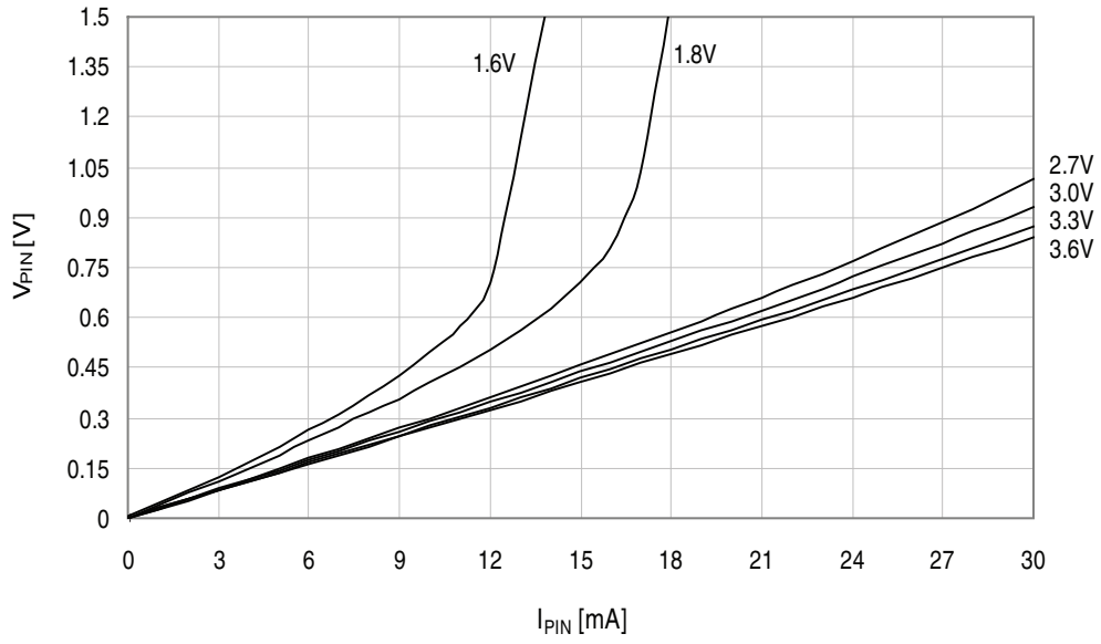
Figure 37-284. I/O pin output voltage vs. sink current.
