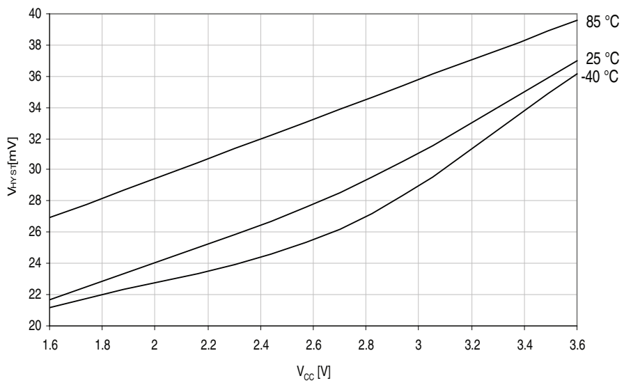
Figure 37-139. Analog comparator hysteresis vs. V_{CC} .
