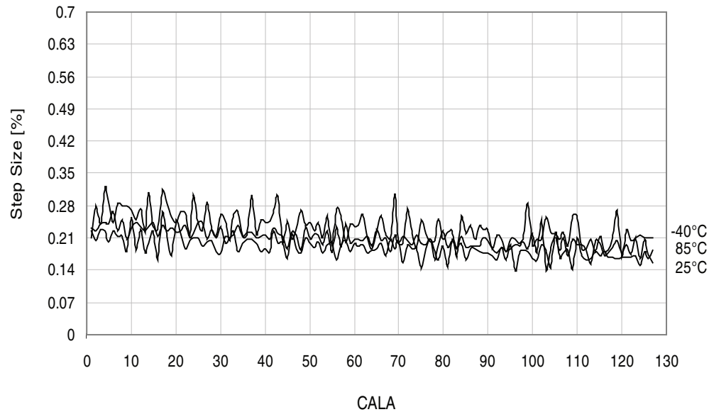
Figure 37-248.32MHz internal oscillator CALA calibration step size.
