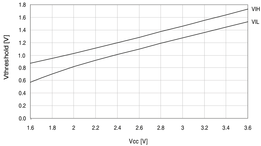
Figure 37-117. I/O pin input threshold voltage vs. V_{CC} . T = 25^{\circ}\text{C} .
