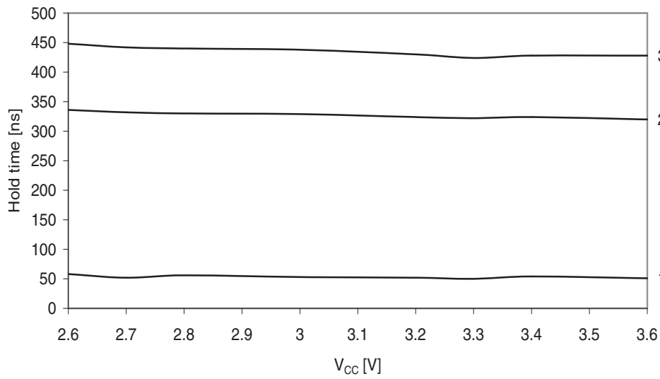
Figure 37-335.SDA hold time vs. supply voltage.
