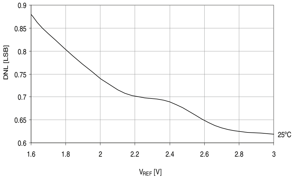
Figure 37-220. DNL error vs. V_{REF} . T = 25^{\circ}C , V_{CC} = 3.6V .
