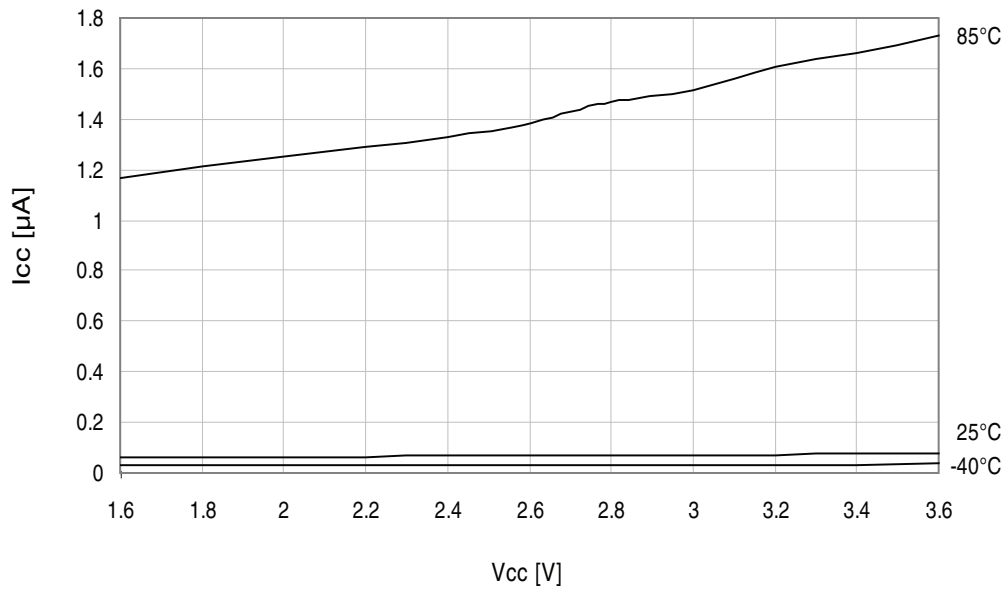
Figure 37-269. Power-down mode supply current vs. V_{CC} . All functions disabled.
