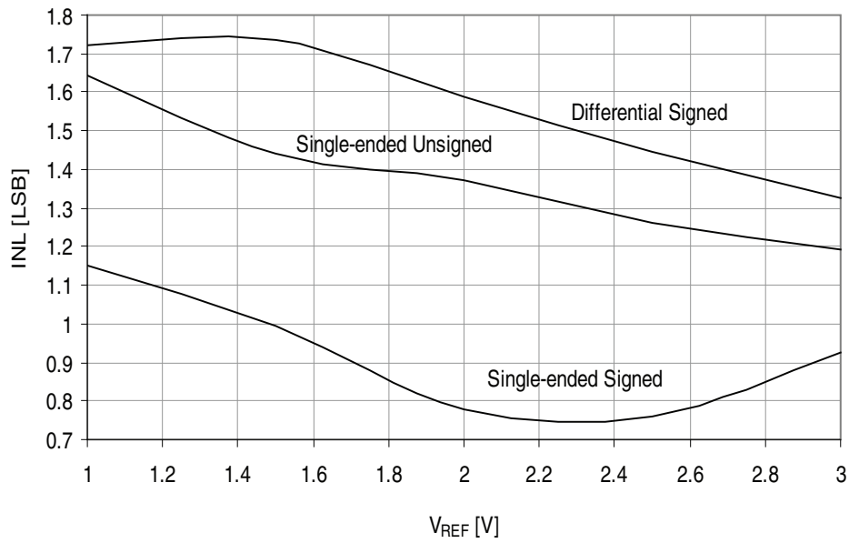
Figure 37-36. INL error vs. external V_{REF} .
