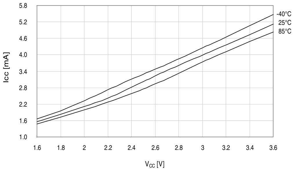
Figure 37-176. Active mode supply current vs. V_{CC} .
