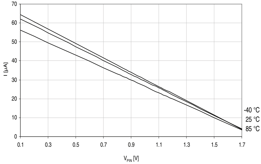
Figure 37-107. I/O pin pull-up resistor current vs. input voltage.
