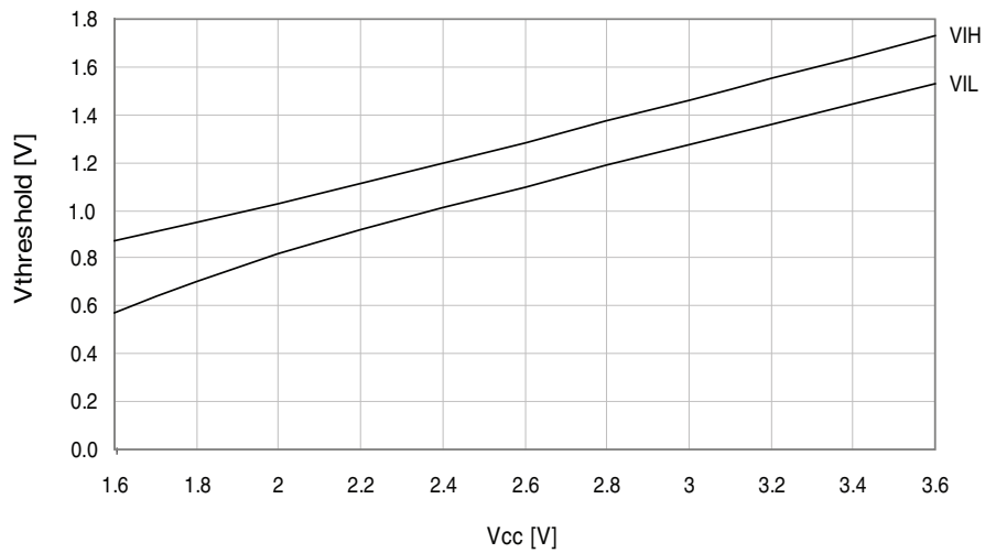
Figure 37-285. I/O pin input threshold voltage vs. V_{CC} . T = 25^{\circ}\text{C} .
