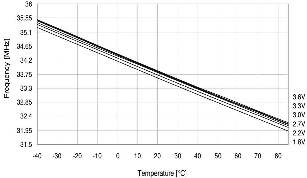
Figure 37-246.32MHz internal oscillator frequency vs. temperature.
