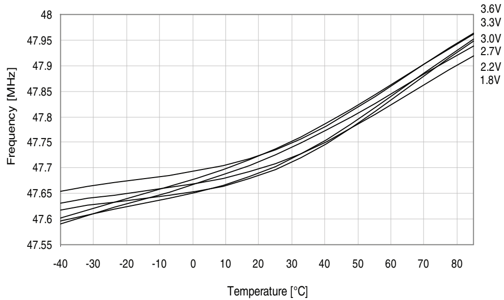
Figure 37-333.48MHz internal oscillator frequency vs. temperature.
