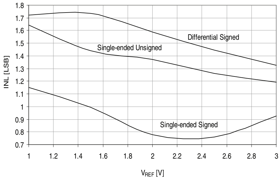
Figure 37-289.INL error vs. external V_{REF} .
