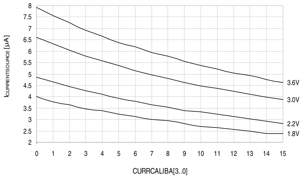
Figure 37-226. Analog comparator current source vs. calibration value.
