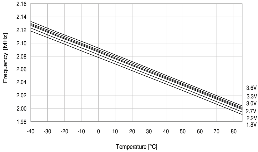
Figure 37-327.2MHz internal oscillator frequency vs. temperature. DPLL enabled, from the 32.768kHz internal oscillator.
