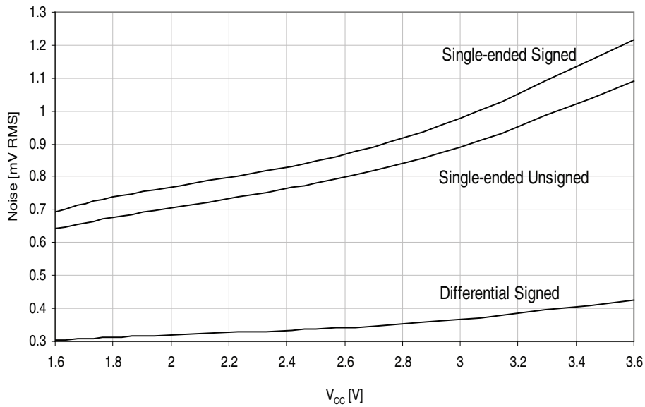
Figure 37-301.Noise vs. V_{CC} .
