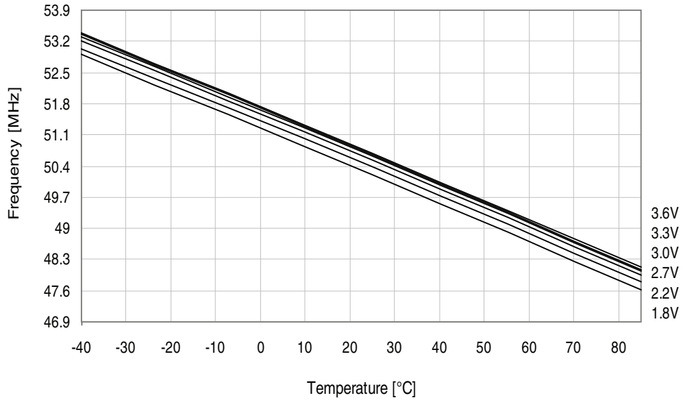
Figure 37-250.48MHz internal oscillator frequency vs. temperature.
