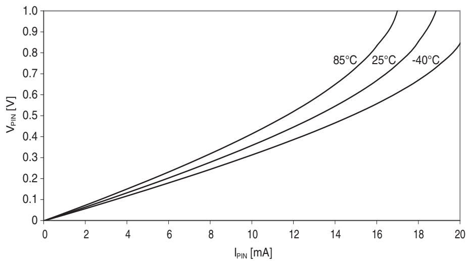
Figure 37-113. I/O pin output voltage vs. sink current.
