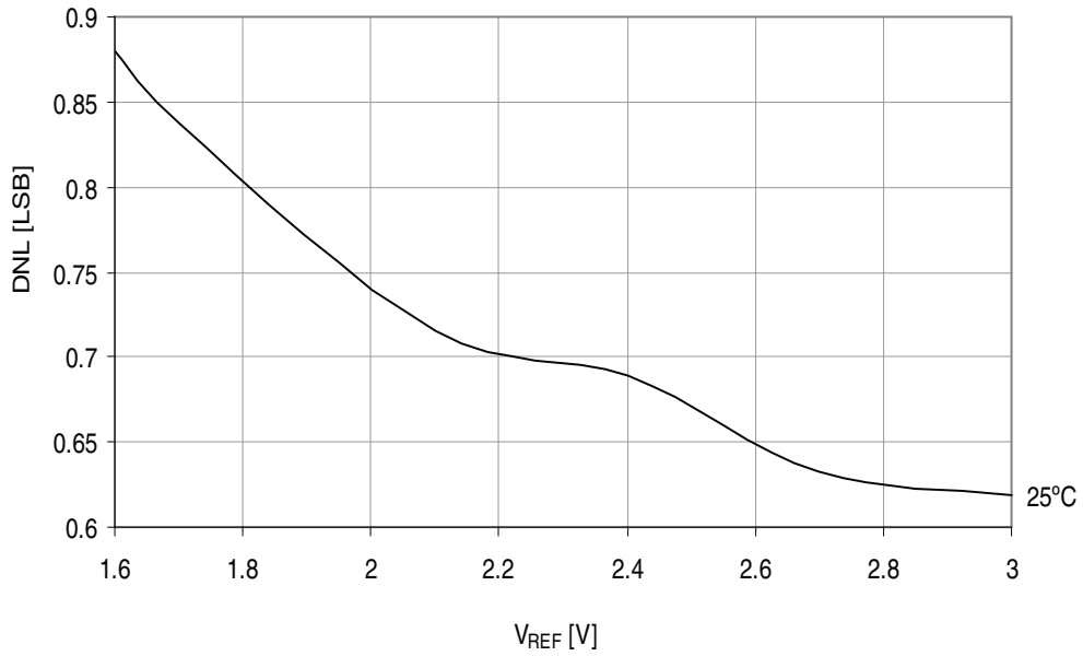
Figure 37-303. DNL error vs. V_{REF} . T = 25^{\circ}C , V_{CC} = 3.6V .
