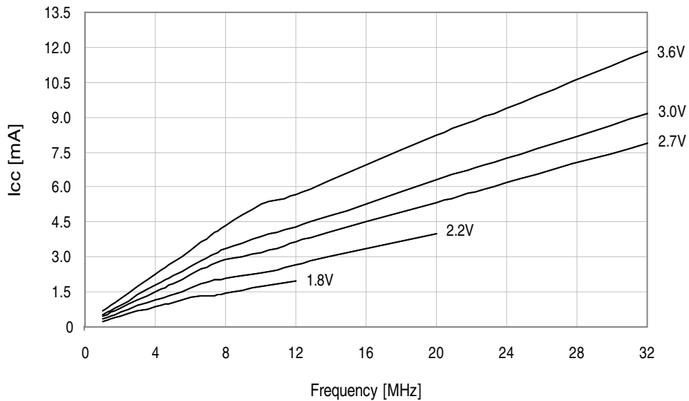
Figure 37-172. Active supply current vs. frequency.
