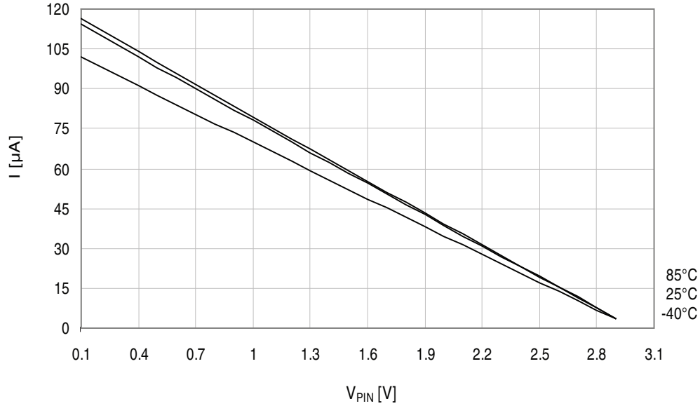
Figure 37-275. I/O pin pull-up resistor current vs. input voltage.
