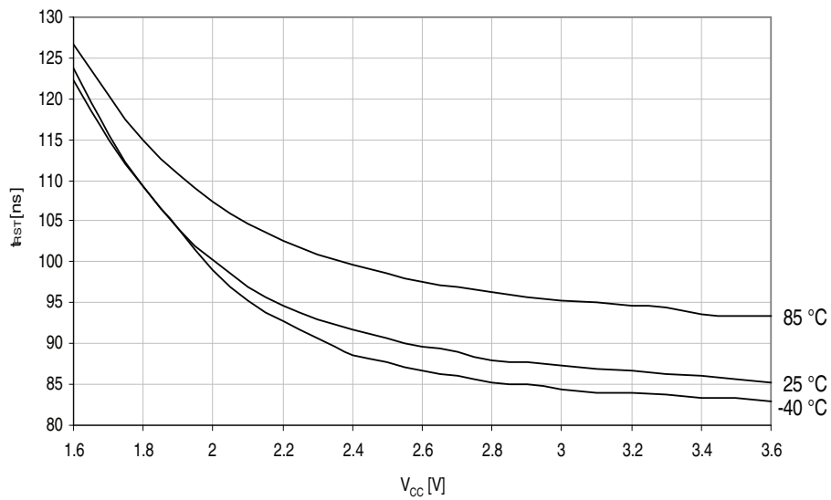
Figure 37-147. Minimum Reset pin pulse width vs. V CC .
