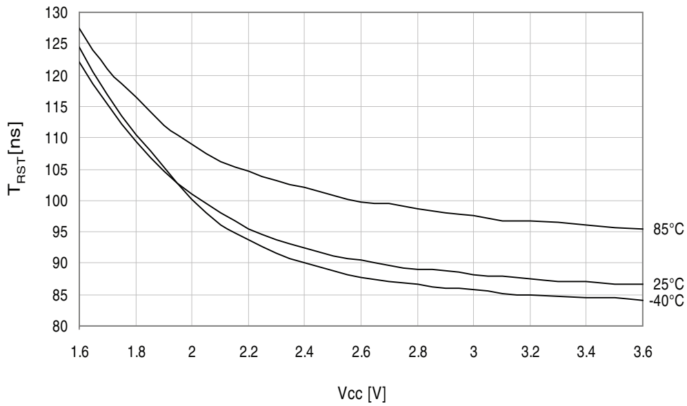
Figure 37-315. Minimum Reset pin pulse width vs. V CC .
