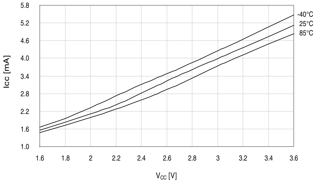
Figure 37-259. Active mode supply current vs. V_{CC} .
