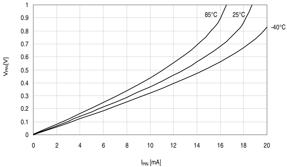
Figure 37-198. I/O pin output voltage vs. sink current.
