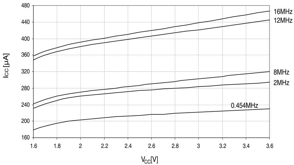
Figure 37-273. Standby supply current vs. V_{CC} . 25°C, running from different crystal oscillators.
