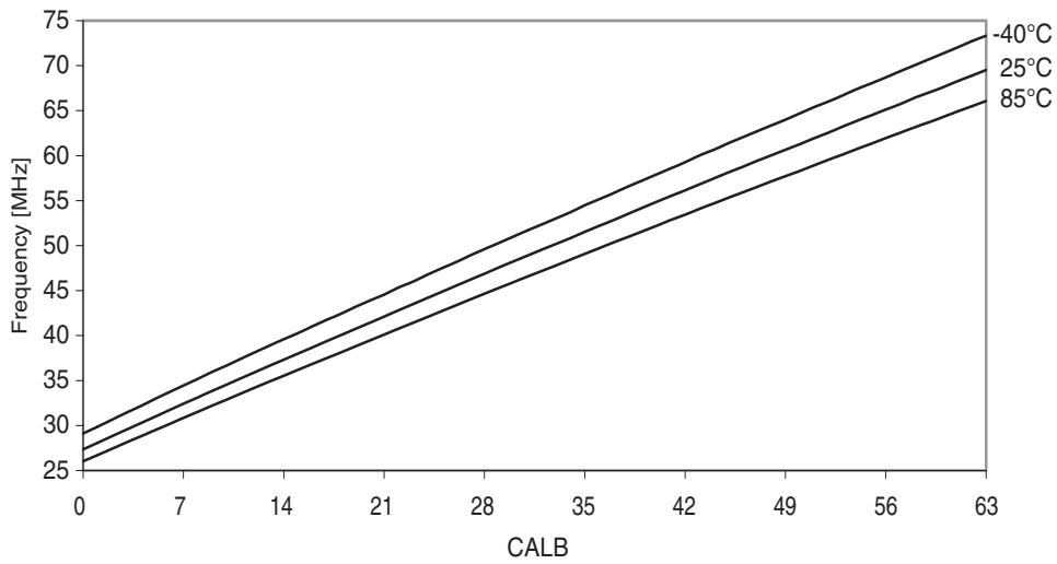
Figure 37-79.32MHz internal oscillator frequency vs. CALB calibration value.
