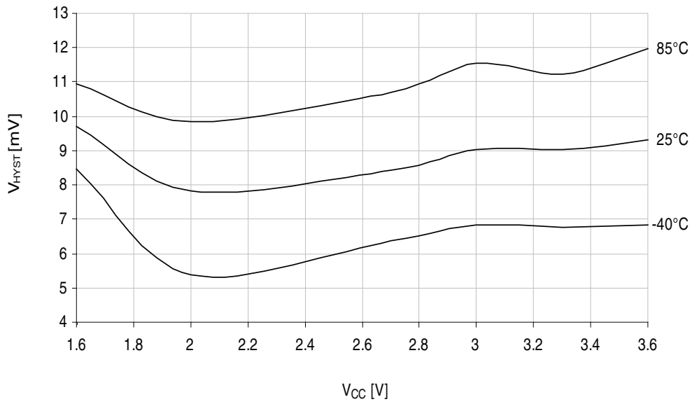
Figure 37-305. Analog comparator hysteresis vs. V_{CC} .
