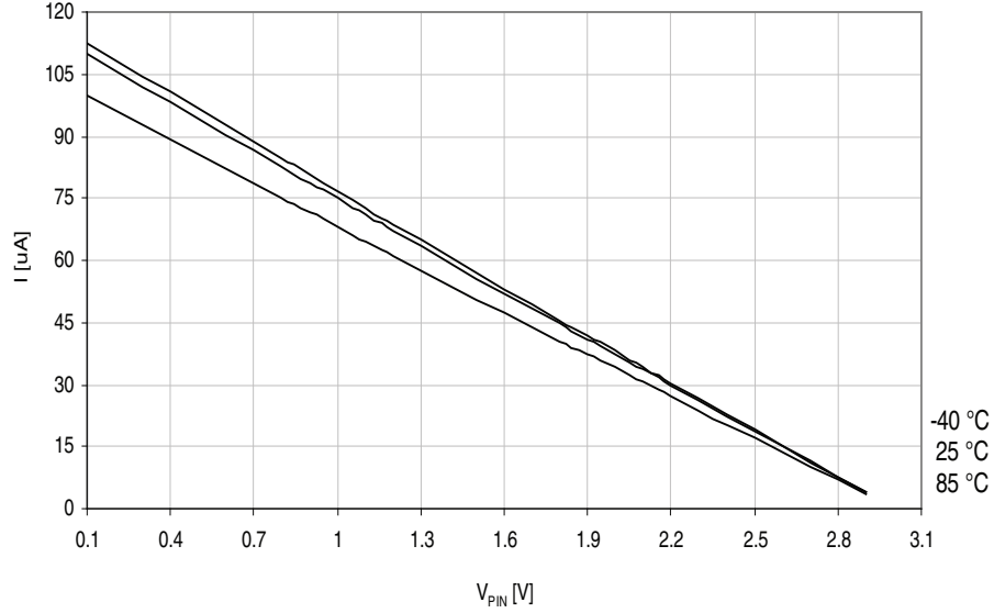
Figure 37-107. I/O pin pull-up resistor current vs. input voltage.
