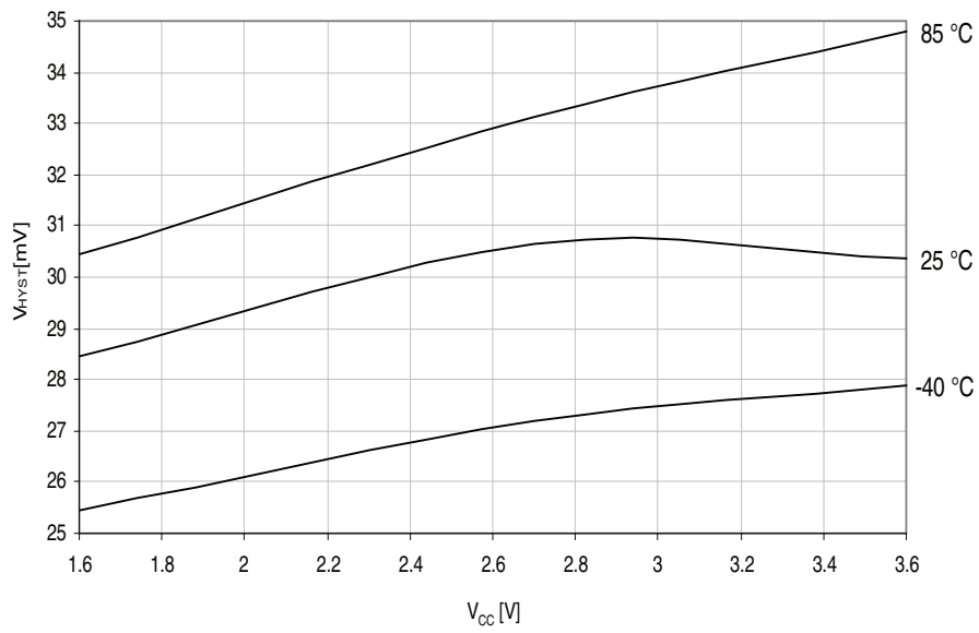
Figure 37-139. Analog comparator hysteresis vs. V_{CC} .
