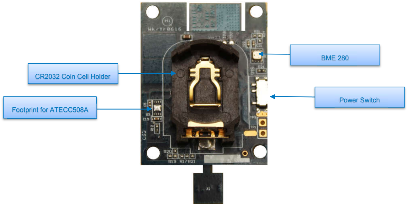
Figure 1-4. Bottom Side
