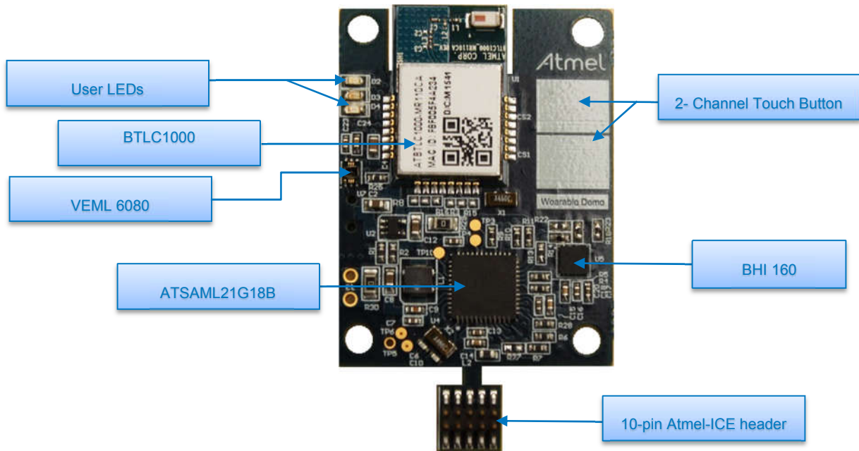
Figure 1-3. Top Side
