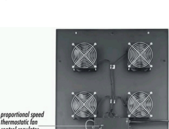
proportional speed thermostatic fan control regulates fan speed proportional to heat inside enclosure
