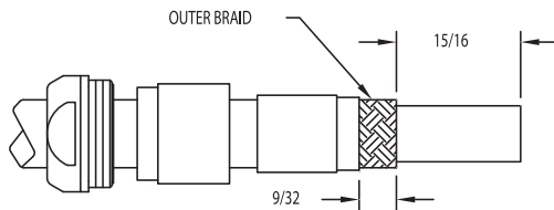
2. REMOVE JACKET AND OUTER BRAID TO 15/16 DIM. THEN REMOVE JACKET AN ADDITIONAL 9/32 EXPOSING OUTER BRAID.
