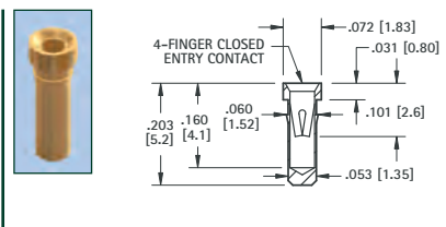
IC SOCKET CONTACTS FOR .015 (.38) - .025 (.64) LEADS - PRESS-FIT
