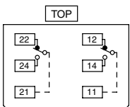
(SPDT contacts on the right only)
