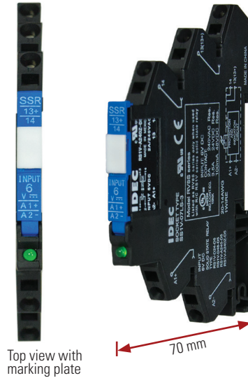
Solid State (spring clamp)
