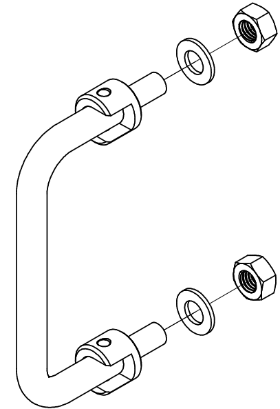
TYPICAL EXPLODED ASSEMBLY
