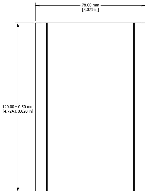
EXTRUSION
