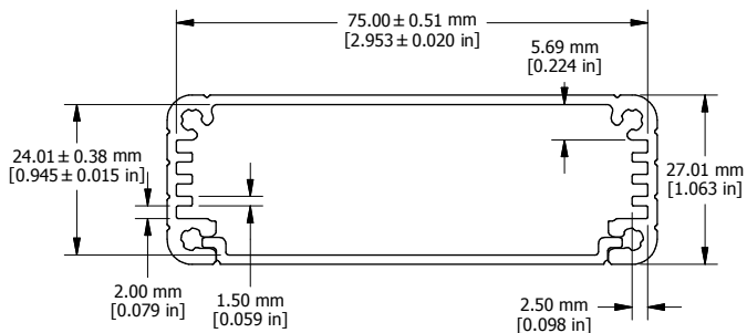
EXTRUSION
