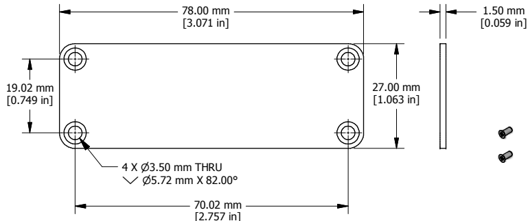
END PLATE
