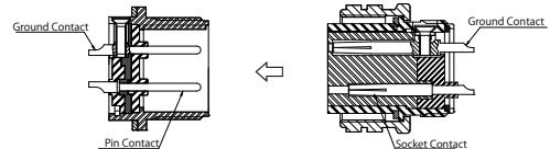
Receptacle Connector
